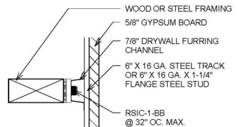
③ ENLARGED DETAIL 3" = 1'-0"
