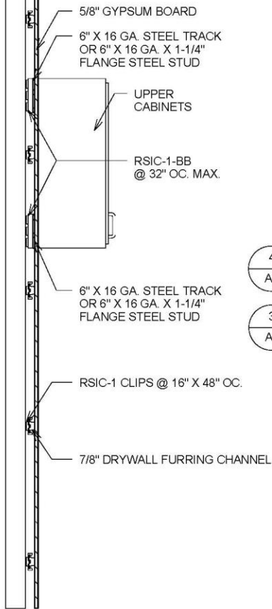
① WALL SECTION 3/4" = 1'-0"
